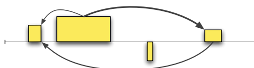
Linked Valued Segments (LVS)
