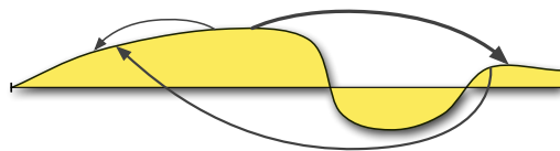
Linked Function (LF)
