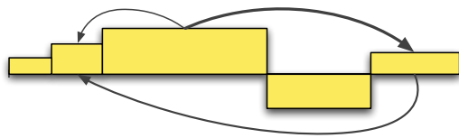
Linked Step Function (LSF)
