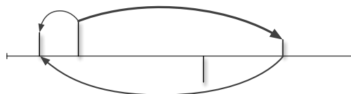
Linked Valued Points (LVP)
